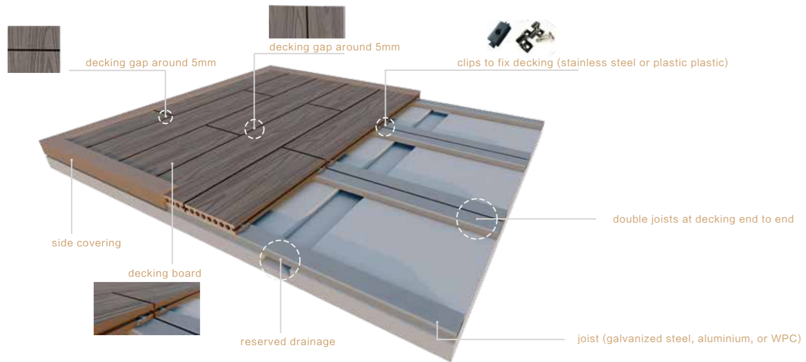
Decking Installation Sketch
